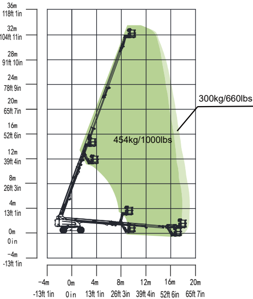
Range of Motion ZT32JE-V
