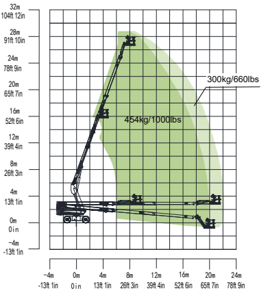
Range of Motion ZT26JE
