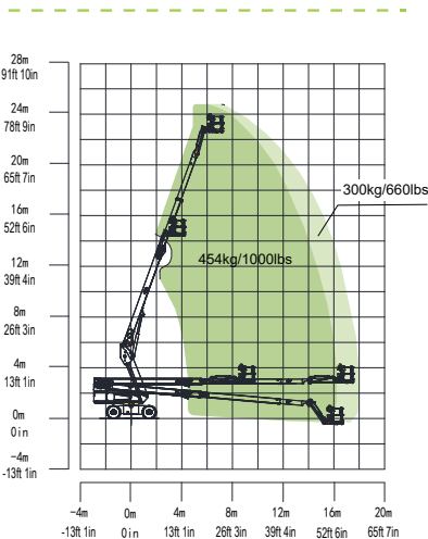
Range of Motion ZT22JE
