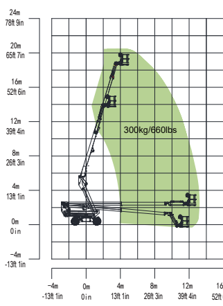
Range of Motion ZT18JE-V (Li)
