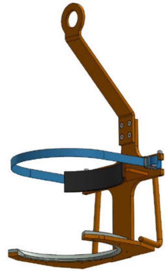
115 601 Loading fork LG 0.4 Carrying capacity 40 kg 115 518 C-hook with counterbalance and storage rack Carrying capacity 15 t Coil width 1.5 m
