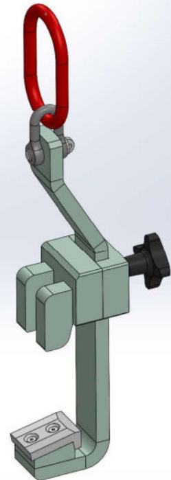
115 652 C-hook CH 0.15 Carrying capacity 150 kg
