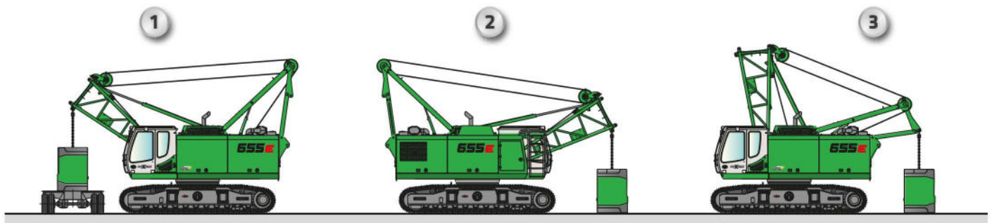
Ballastmontagesystem ballast assembly system
